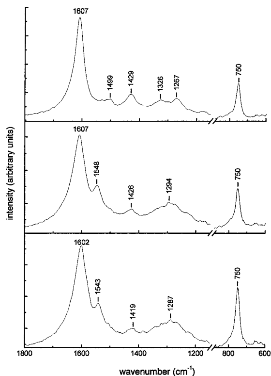
FIGURE 4 UV Raman spectra of novobiocin (a) at pH 7, (b) at pH 11, and (c) in methanol.
